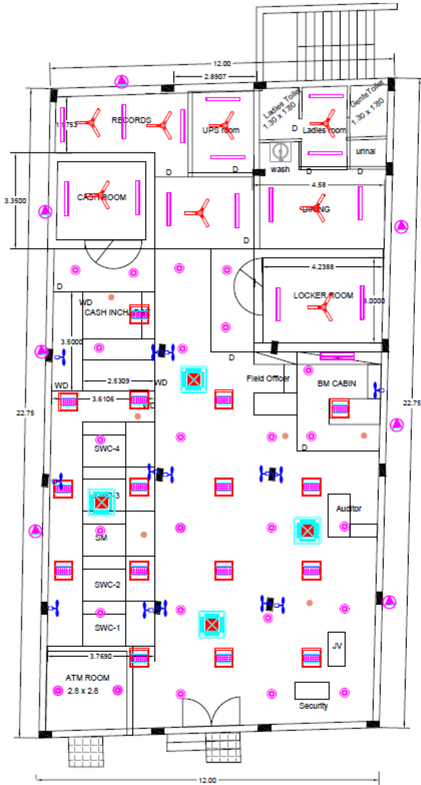
SBI PONGNAD BRANCH - GROUND FLOOR PLAN DRAWING NO.1 DATED 23.05.23
